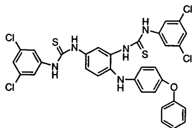
Compound # 40
